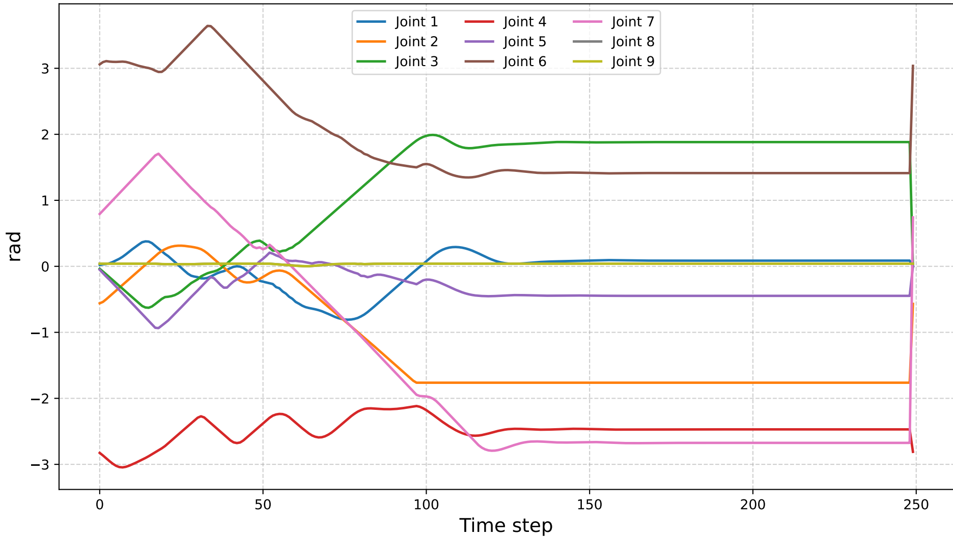
Joint Positions
