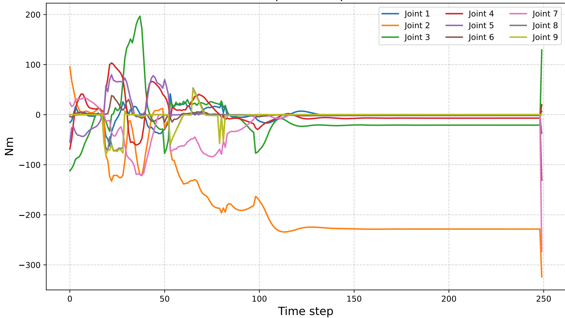
Computed Torques
