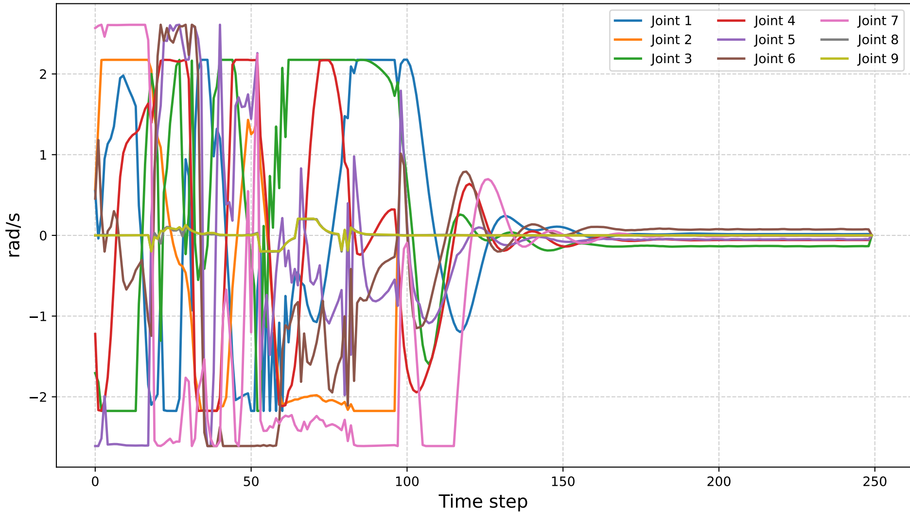
Joint Velocities
